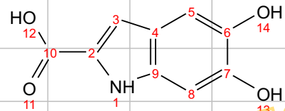
5,6-Dihydroxy-1H-indole-2-carboxylic acid CAS:4790-08-3
